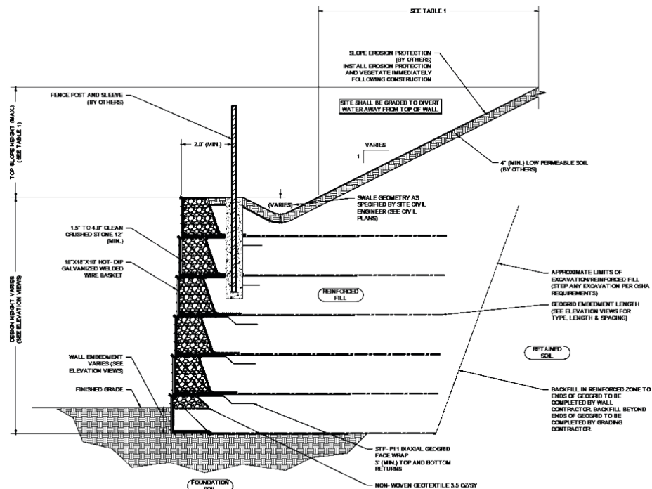
TYPICAL CROSS SECTION - TOP SLOPE SCALE: 1:20
