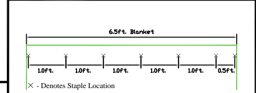
Figure D - Plan View x - Denotes Staple Location
